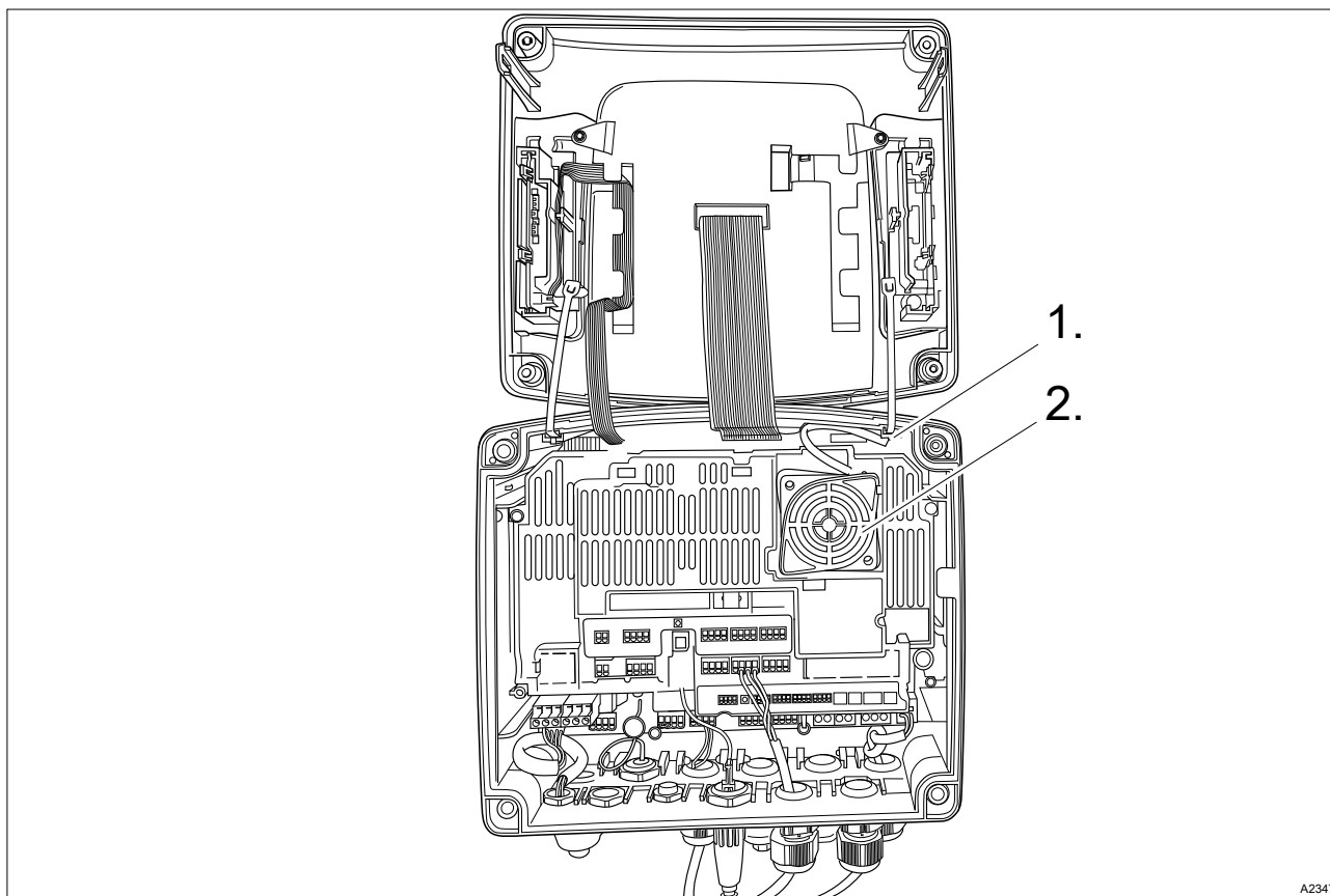
Fig. 131: Replacing fan, part no. 733328
