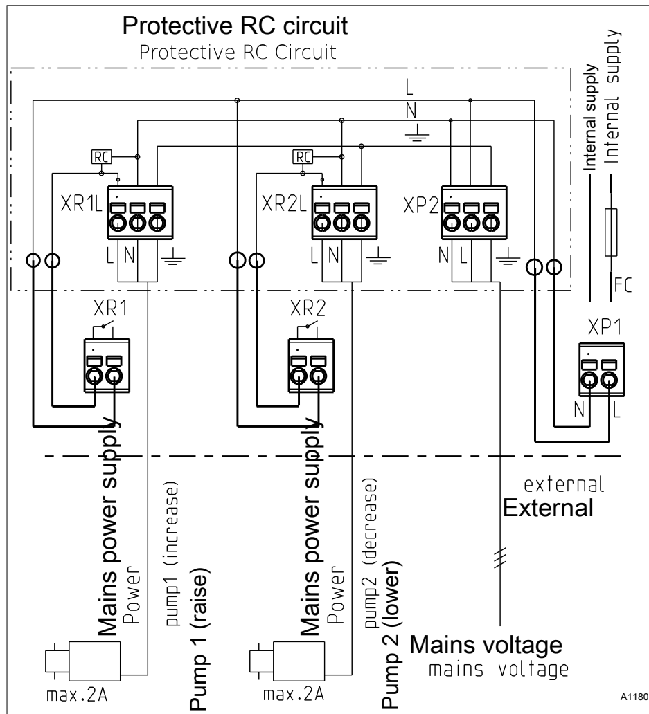
Fig. 22: Terminal diagram with protective RC circuit (module D, optional). The RC unit is only permitted in conjunction with the 230 V design.
