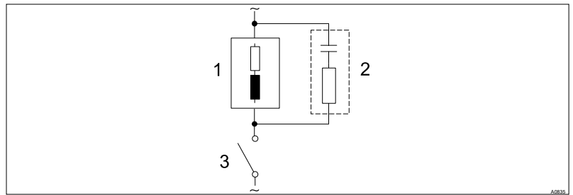
Fig. 30: RC protective circuit for the relay contacts
