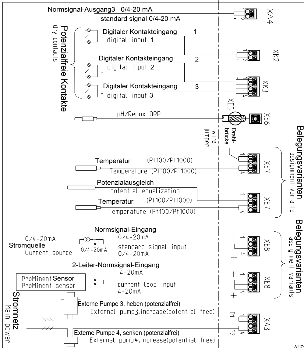
Fig. 21: Terminal diagram for the extension unit (channel 3) with assignment options (module C, optional)
