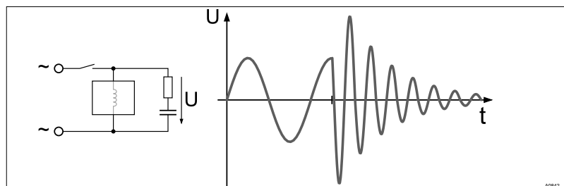
Fig. 29: Switching-off process shown on the oscillogram.
