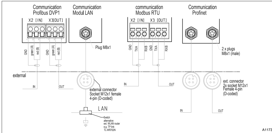
Fig. 23: Terminal diagram for the DAC communication unit (module B, optional)
