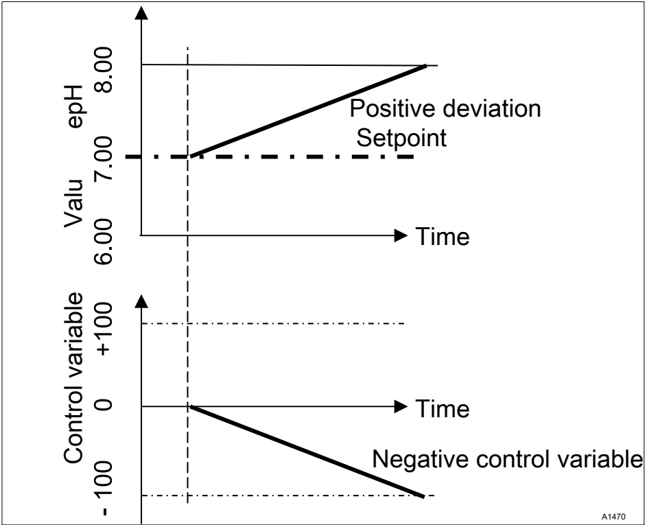
Fig. 89: Control type PID monodirectional, pH-lowering direction
