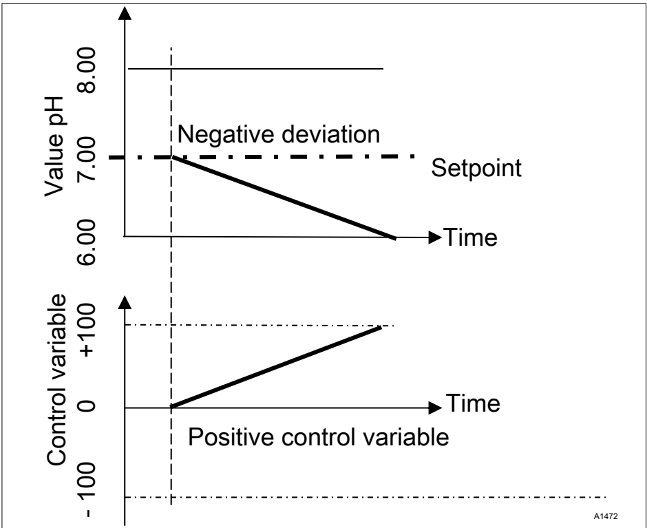
Fig. 90: Control type PID monodirectional, pH-raising direction
