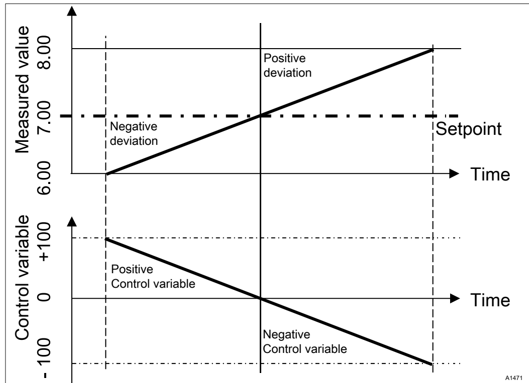
Fig. 87: Control type PID bidirectional. Control characteristic without neutral zone
