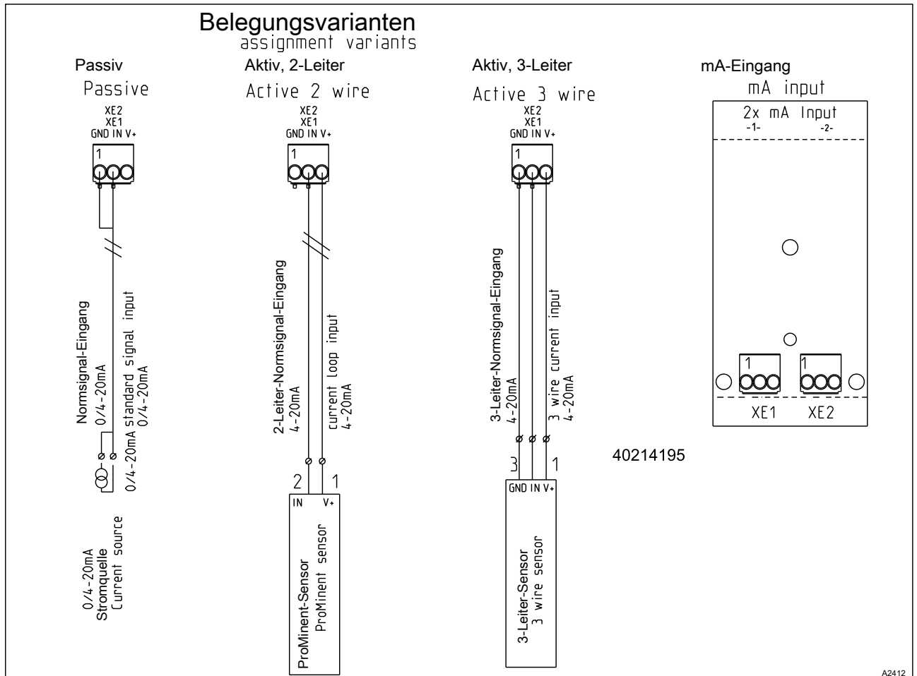
Fig. 28: Module: 2x mA inputs. Part number 734126
