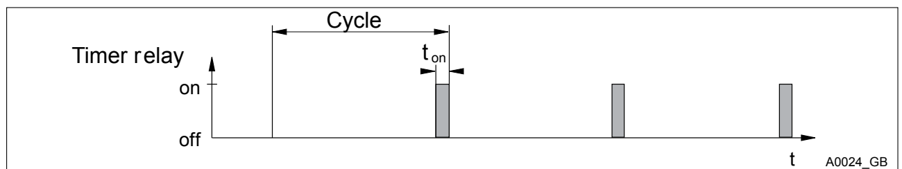
Fig. 107: Timer relay
