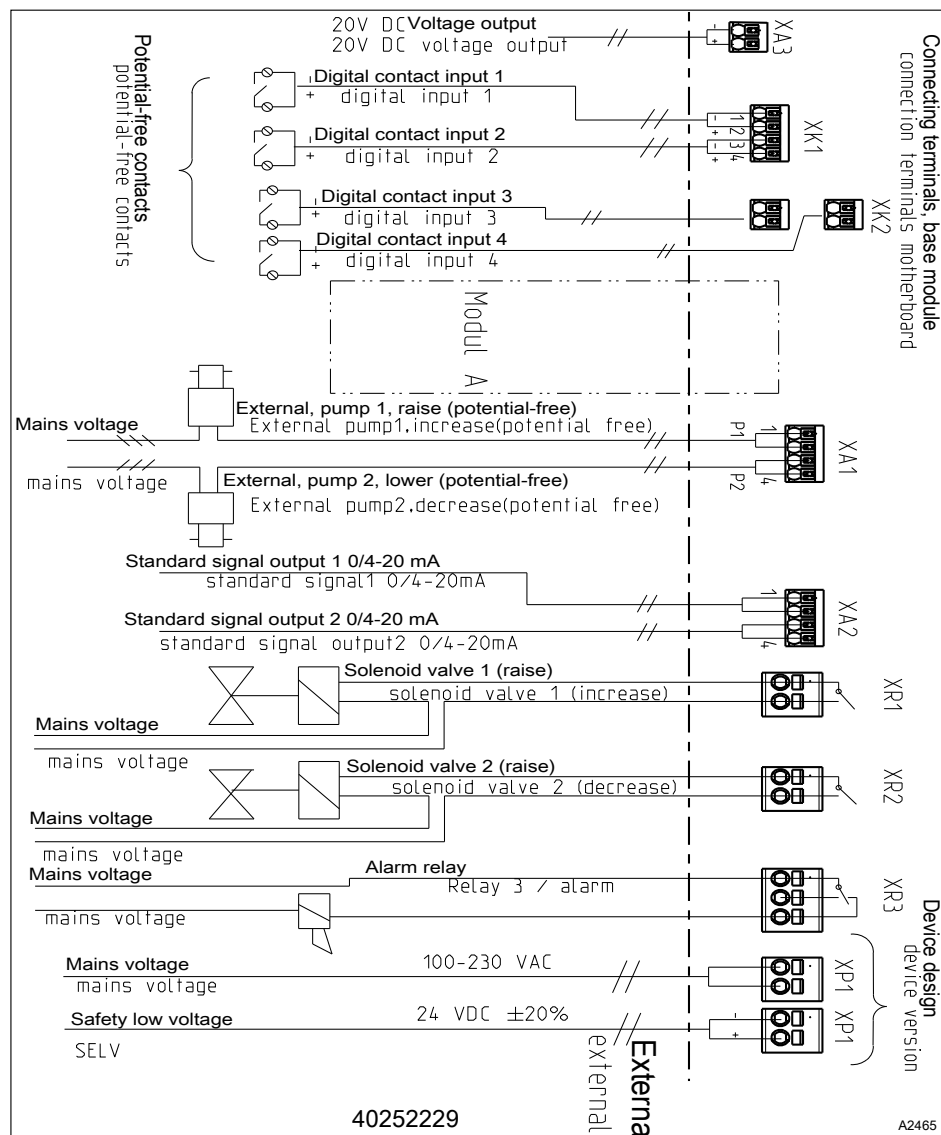
Fig. 20: Terminal diagram with assignment options.
