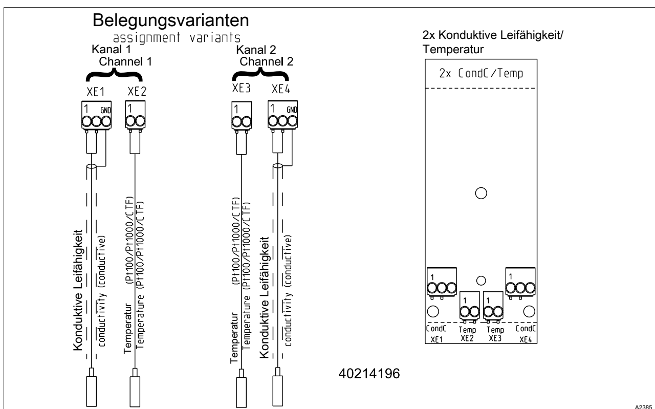
Fig. 27: Module: 2x conductive conductivity/temperature sensors. Part number 734223
