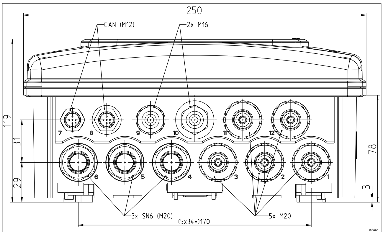
Fig. 16: All dimensions in millimetres (mm).
