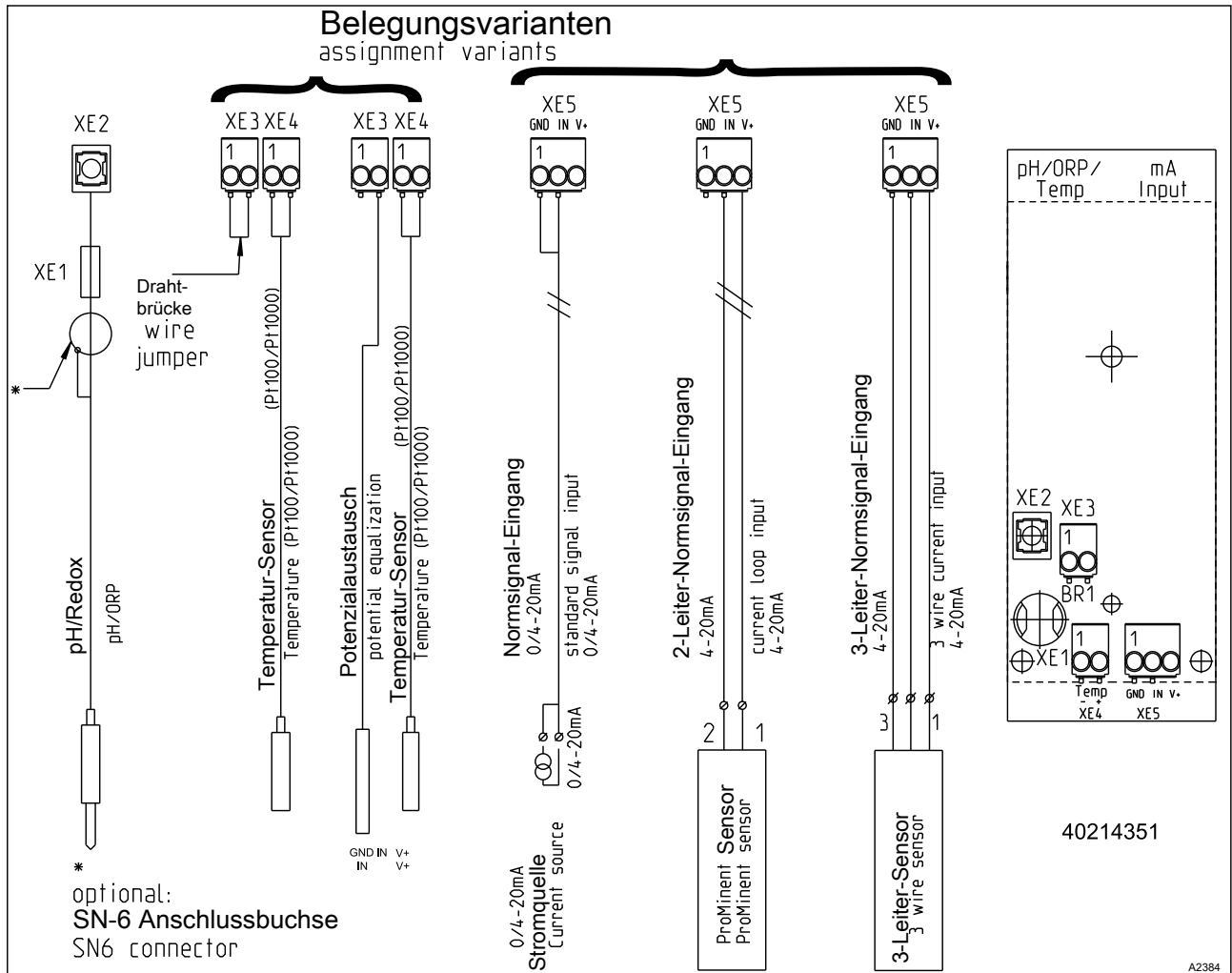
Fig. 25: Module: mV temperature/mA input. Part number 734355
