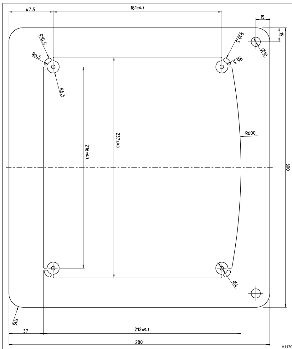
Fig. 15: The drawing is not true to scale and will not be updated as part of these operating instructions. The drawing is for information only.
