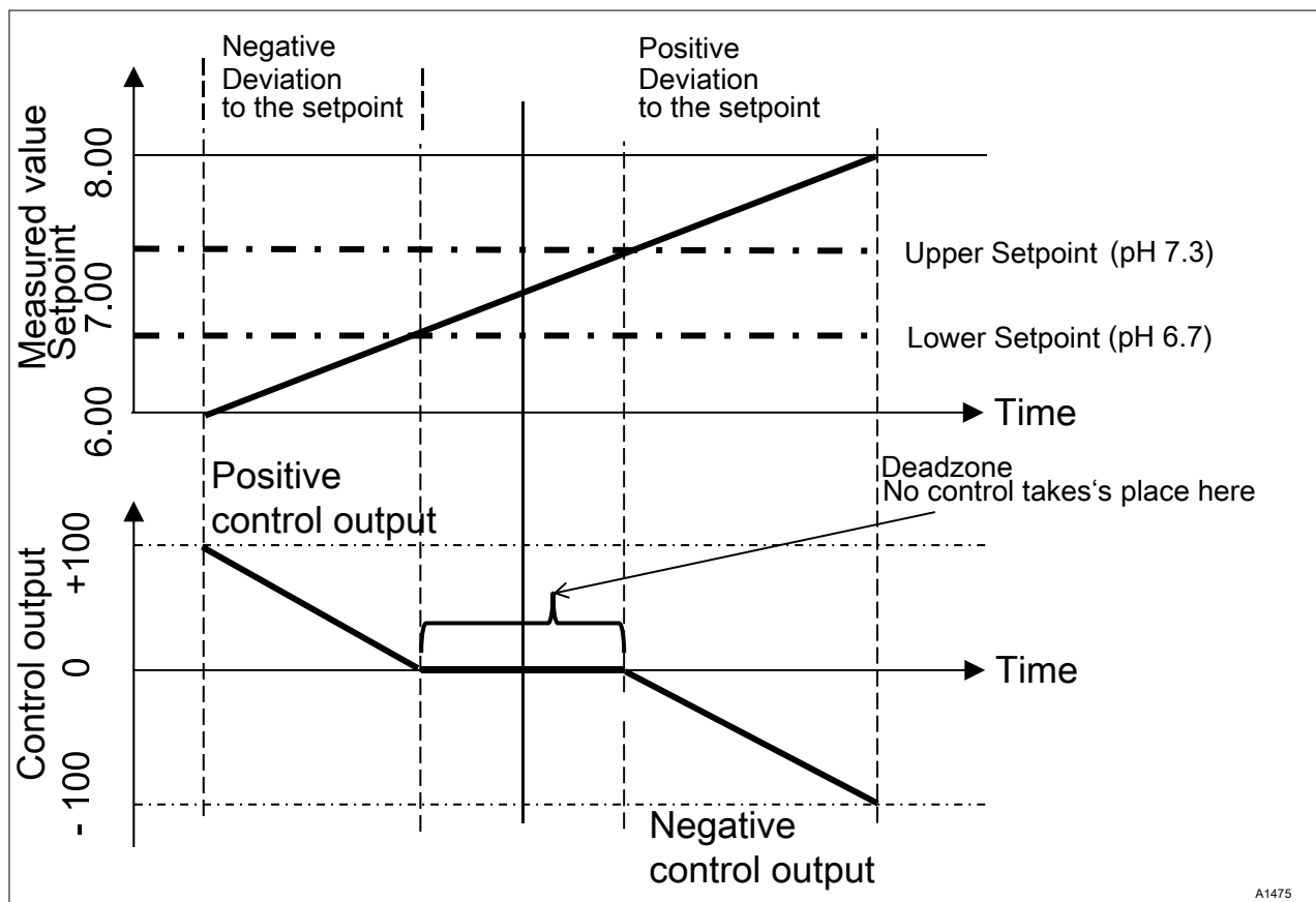
Fig. 88: Control type PID bidirectional, with neutral zone
