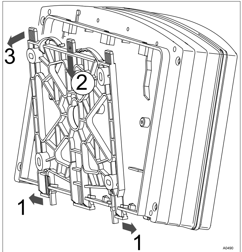
Fig. 11: Dismantling surface mount
