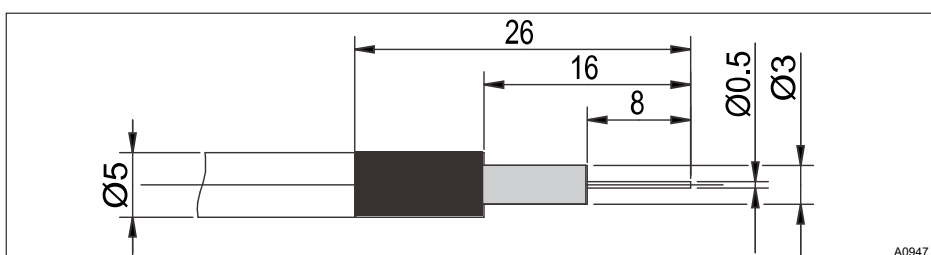
Fig. 32: Coaxial cable construction
