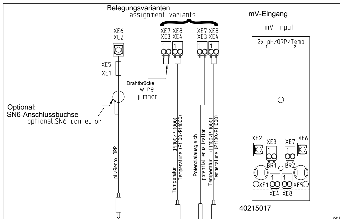
Fig. 26: Module: 2x mV inputs/temperature input. Part number 734131
