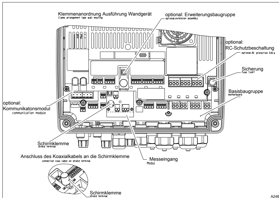
Fig. 19: Terminal layout
