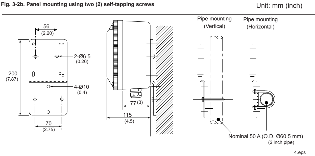
Figure 3-3. Wall and pipe mounting diagram
