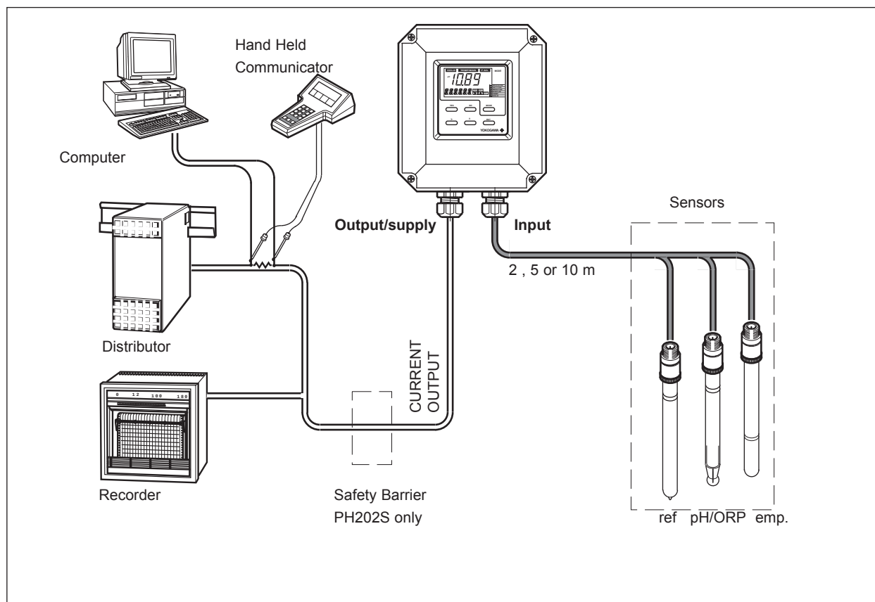
Figure 3-6. System configuration
