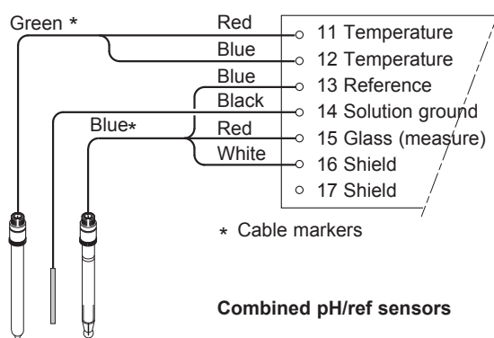
Figure 3-10a. Sensor wiring
