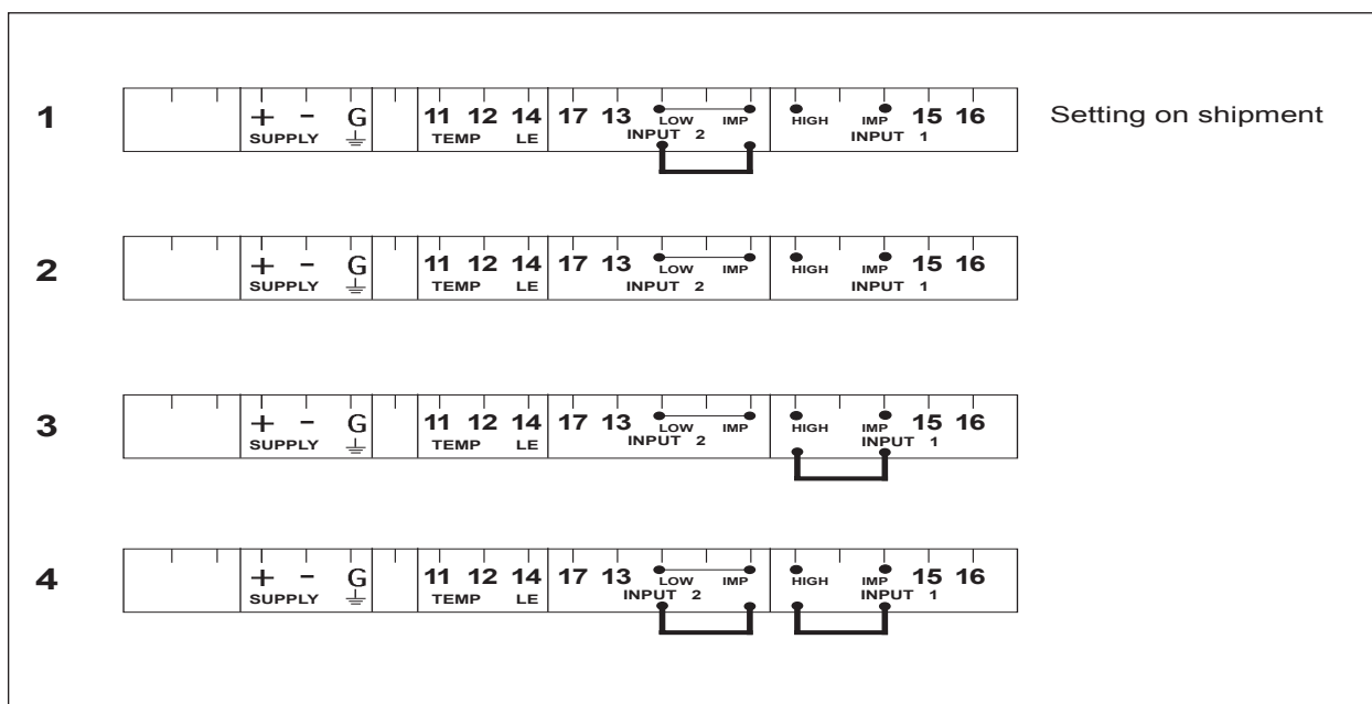
Fig. 3-8. Jumper positions
