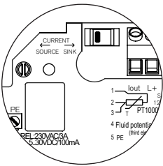
Fig. 3.5 Using switch 1
