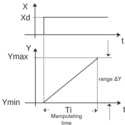
Step response
