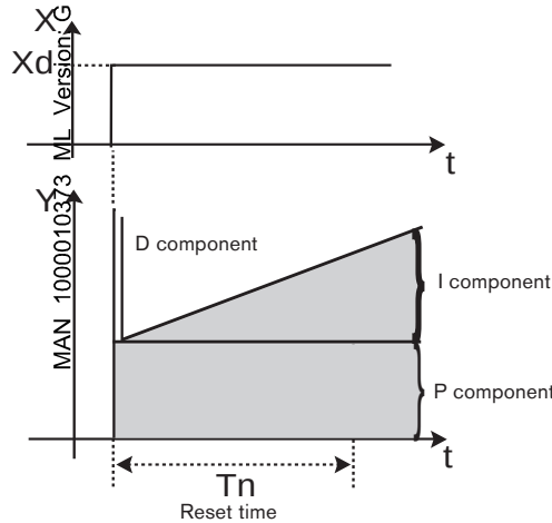
Step response of the PID controller
