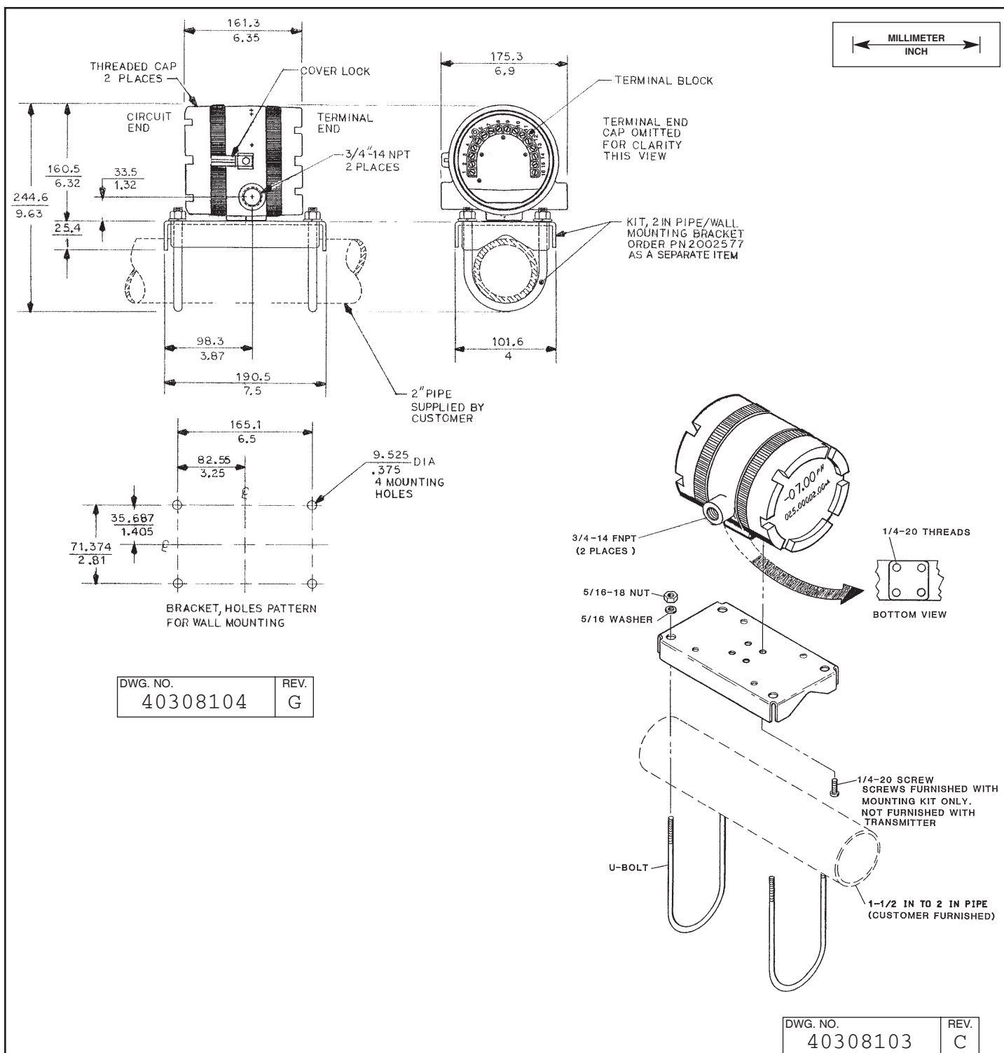
FIGURE 2-5. Using the Pipe Mounting Kit to Attach the Model 4081 pH/ORP Transmitter to a Pipe
