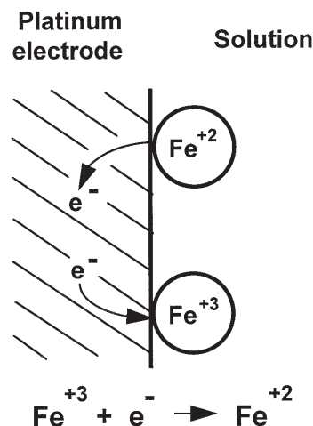
FIGURE 13-5. Electrode Potential.
