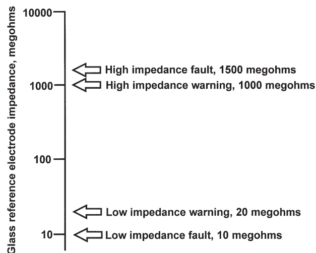
FIGURE 9-2. Suggested Glass Impedance Warning and Failure Limits for a Glass Reference Electrode
