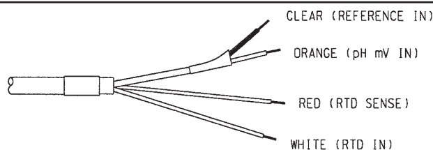
FIGURE 3-2. Wire functions for Models 399-02, 399-09, 381pH-30-41, and 381pHE-31-41 before removing BNC and terminating cable.
