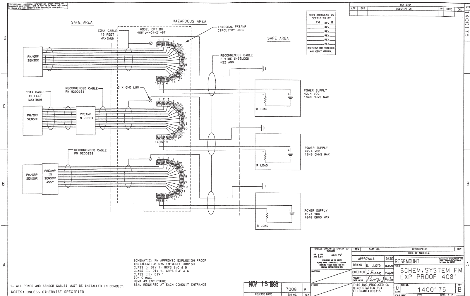
FIGURE 4-2. FM Explosion-Proof Installation for Model 4081 pH/ORP Transmitter
