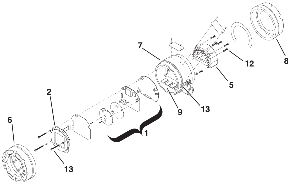
FIGURE 10-1. Exploded View of Model 4081 pH/ORP Transmitter
