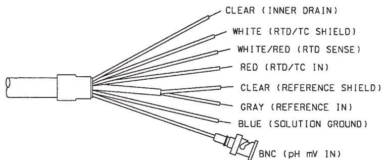
FIGURE 3-15. Wire functions for Model 385+ -02.
