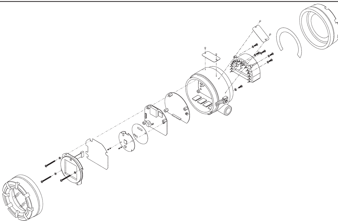
FIGURE 2-1. Model 4081 pH/ORP Transmitter - Exploded Drawing of Circuit Board Stack
