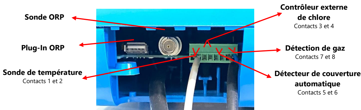
Figure 6 - Connexions internes
