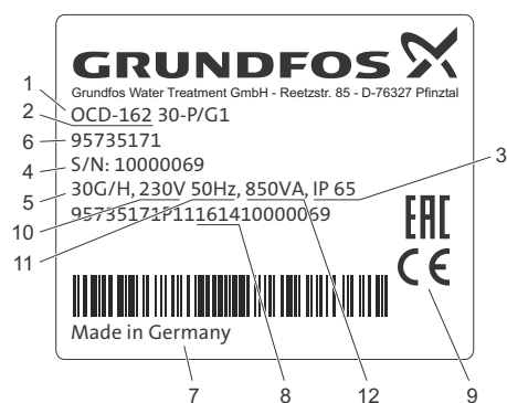
Fig. 2 Nameplate
