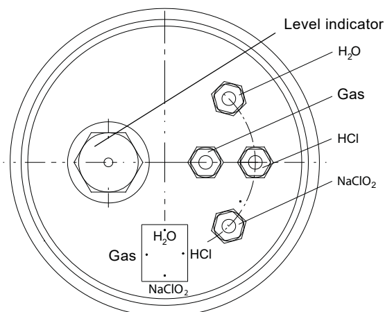
Fig. 40 OCD-162-5, -10: connections on the reaction tank
