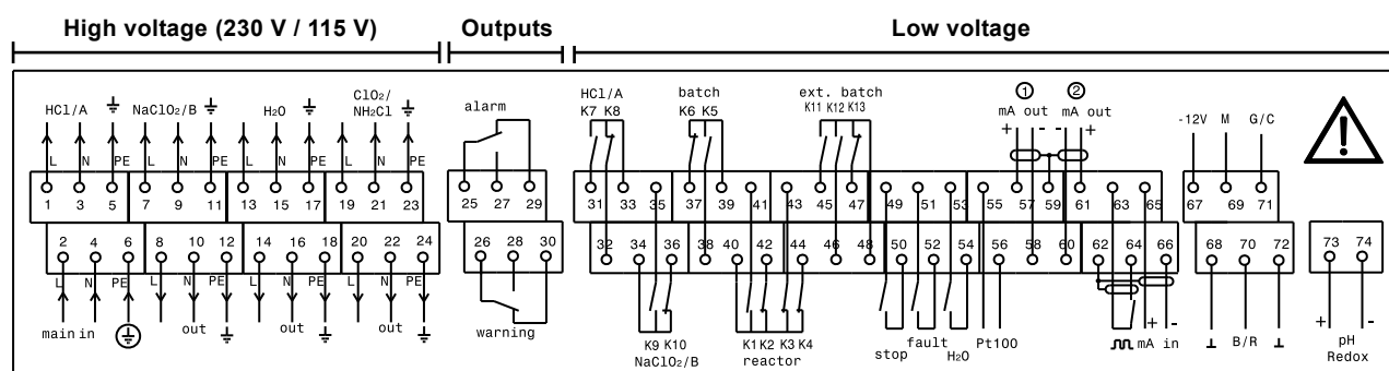
Fig. 48 Terminal connection plan
