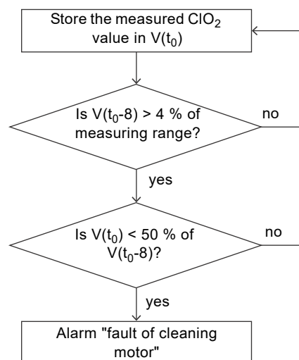
Fig. 15 Process of monitoring the cleaning motor
