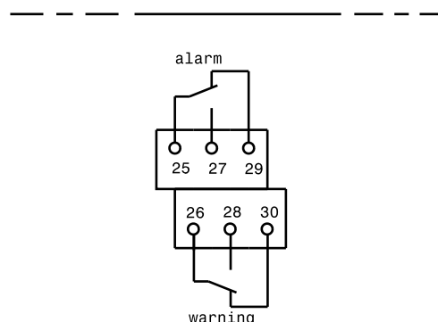
Fig. 50 Terminal connection plan - middle section
