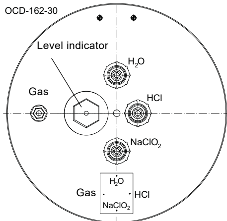
Fig. 41 OCD-162-30: connections on the reaction tank
