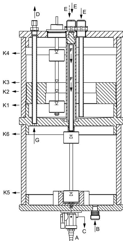
Fig. 8 Reaction tank and internal batch tank (OCD-162-5/-10/-30)
