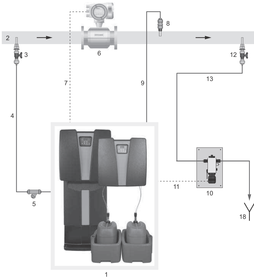
Fig. 3 OCD-162 with measuring cell
