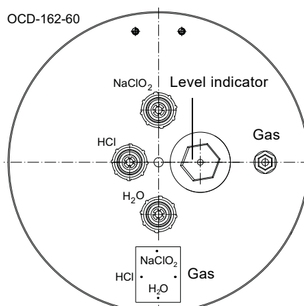
Fig. 42 OCD-162-60: connections on the reaction tank
