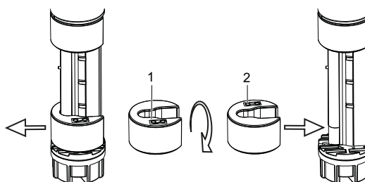
Fig. 22 Reversing the floater
