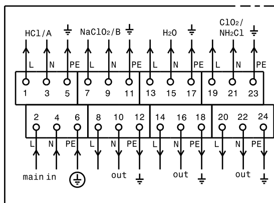
Fig. 49 Terminal connection plan - left section
