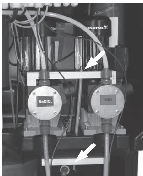
Fig. 18 Transport protection of OCD-162-60
