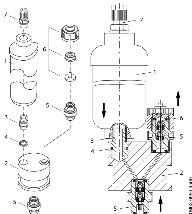
Fig. 45 Maintaining the activated carbon filter
