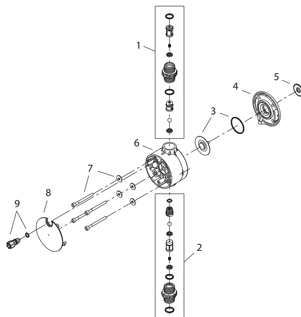
Fig. 35 Dosing head of DDE: exploded view
