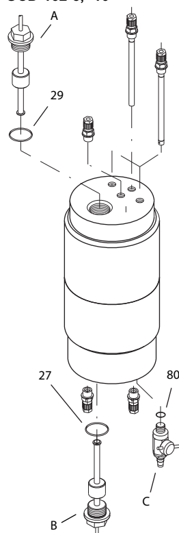
Fig. 43 OCD-162-5, -10, -30: reaction tank/internal batch tank
