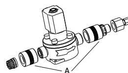
Fig. 37 Solenoid valve OCD-162-05, -10: exploded view
