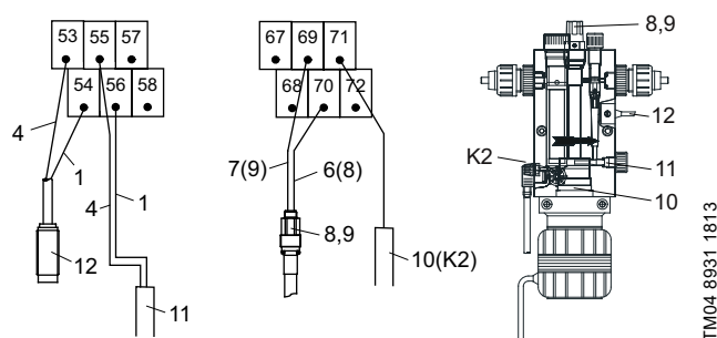
Fig. 27 Connection plan AQC-D1/-D11
