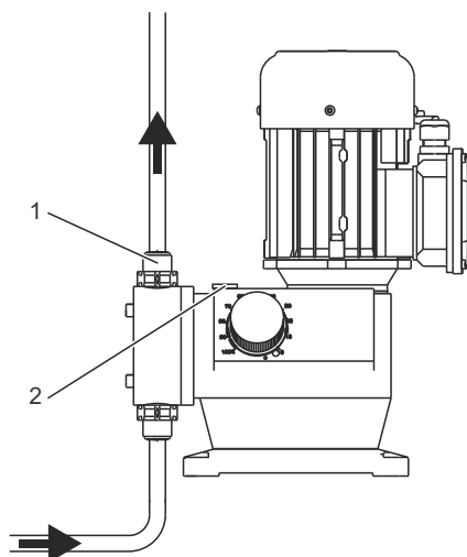
Fig. 21 DMX 35-10 pump
