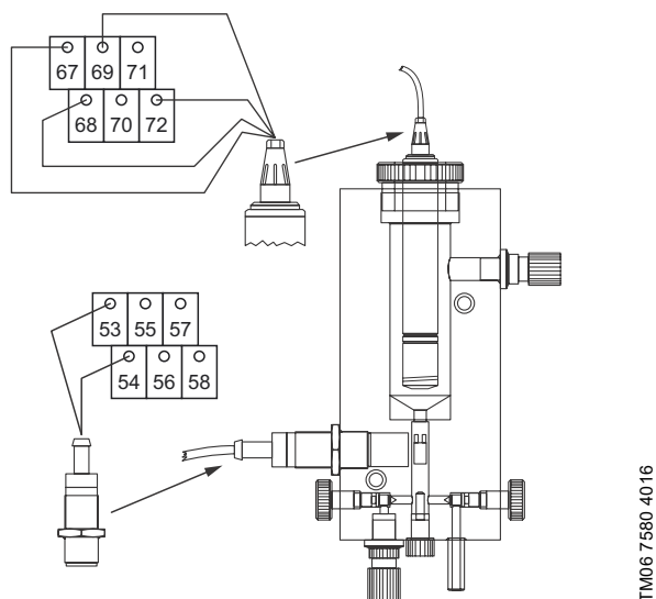
Fig. 28 Connection plan AQC-D6
