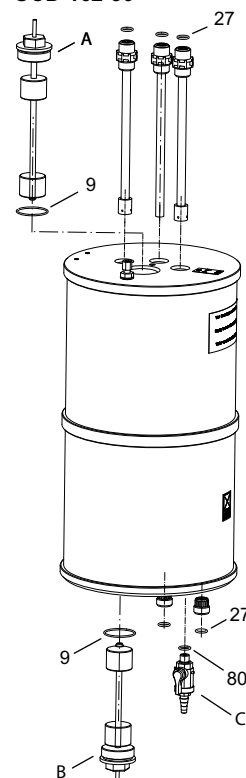
Fig. 43 OCD-162-5, -10, -30: reaction tank/internal batch tank
