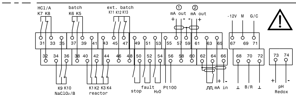
Fig. 51 Terminal connection plan - right section
