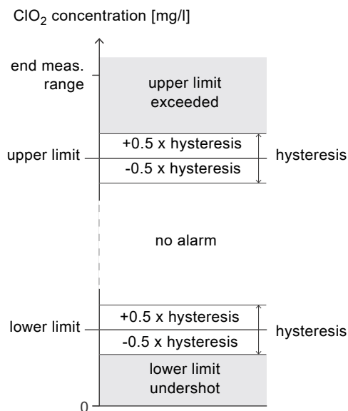
Fig. 16 Alarm limits
