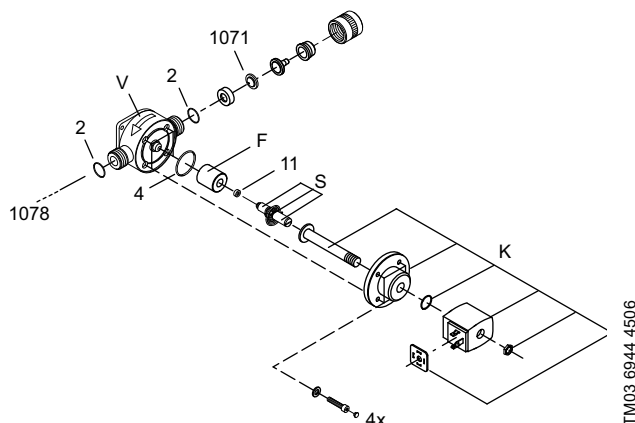
Fig. 36 Solenoid valve (OCD-162-5, -10): exploded view
