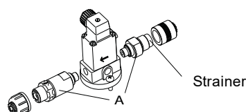
Fig. 38 Solenoid valve OCD-162-30, -60: exploded view
