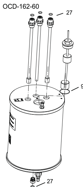
Fig. 44 OCD 162-60: reaction tank
