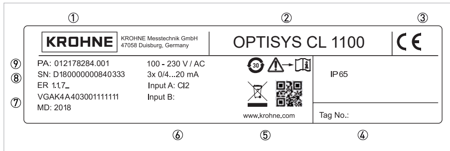
Figure 2-5: Example for a nameplate
