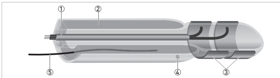
Figure 2-4: Inner parts of the sensor
