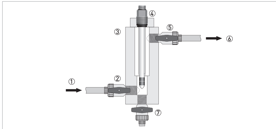
Figure 3-1: Measuring point using the flow cell of the OPTISYS CL 1100 measuring system
