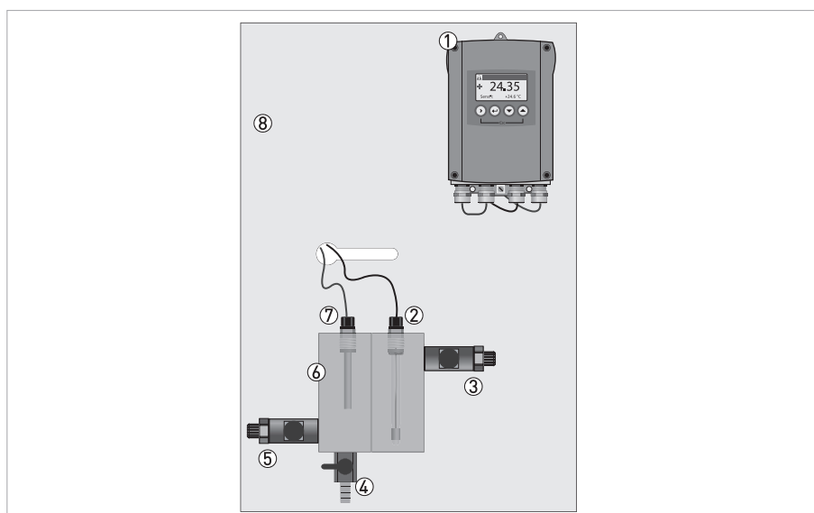
Figure 2-2: Dimension of OPTISYS CL 1100
