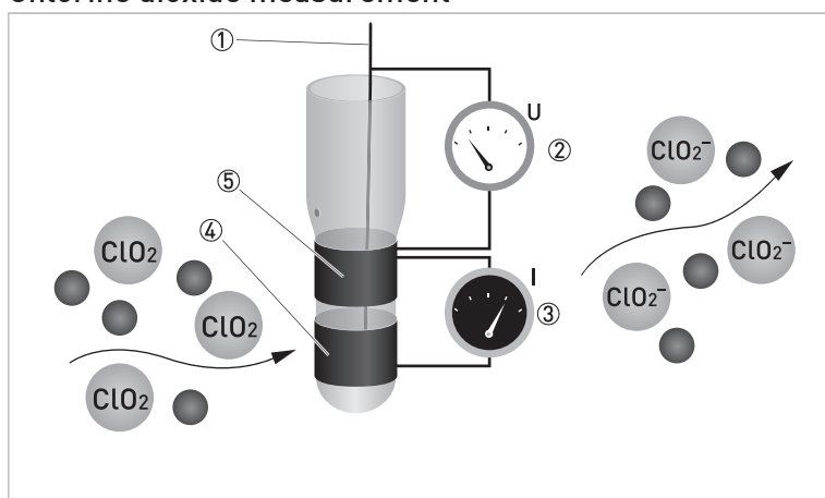
Figure 7-3: Chlorine dioxide measurement
