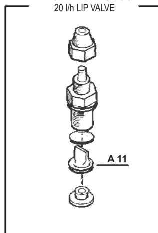
VALVOLA A LABBRO 20 l/h 20 l/h LIP VALVE
