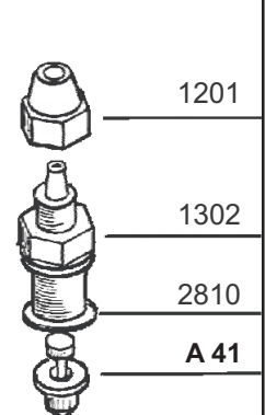
VALVOLA KALRETZ KALRETZ VALVE
