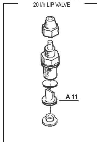
VALVOLA A LABBRO 20 l/h 20 l/h LIP VALVE
