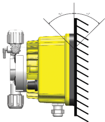
Picture7 Pump Correct Assembly Position
