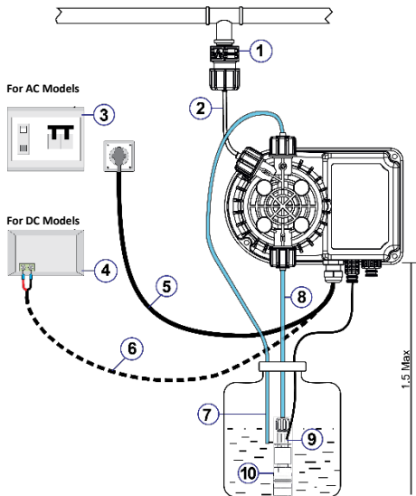
Picture 12 General Assembly for Digital Models
