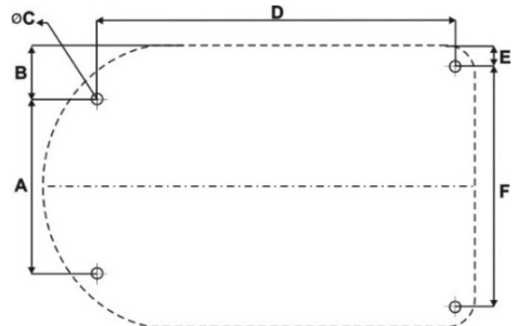
Picture 3 Lara Series Pump Assembly Hole Sizes
