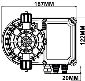
Picture 2 Lara Series Pump Size Front Part
