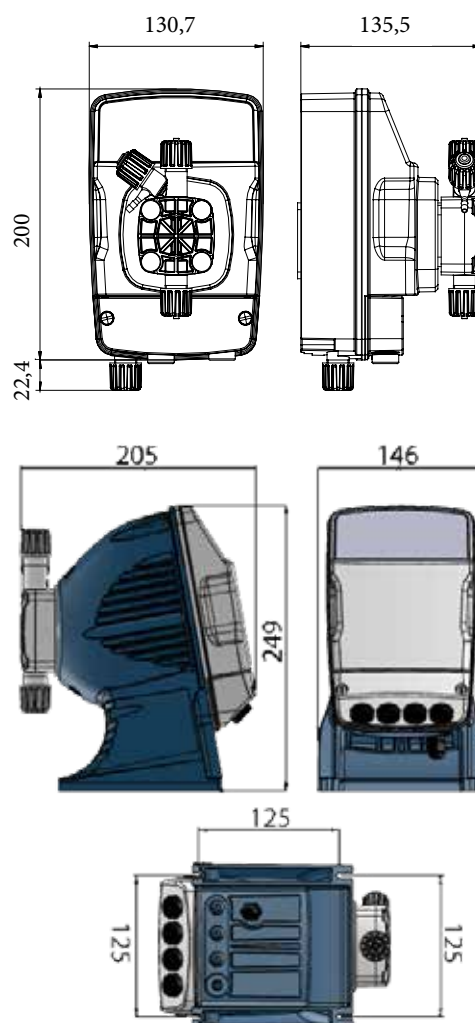
Overall Dimensions
