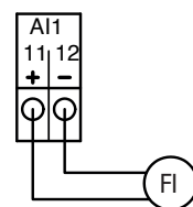
Fig. 32: Flow disturbance variable 4 – 20 mA
