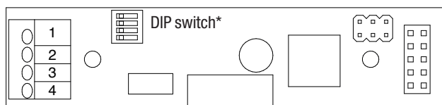
Fig. 20: Conductive input circuit board to the conductivity module
