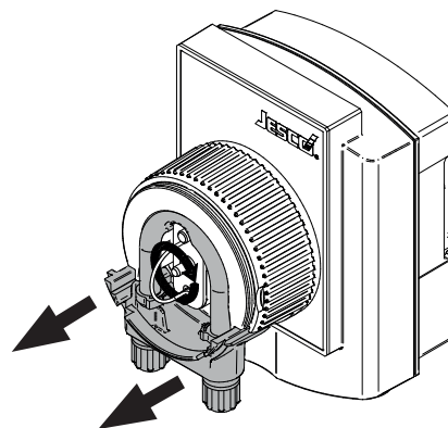
Fig. 49: Hose replacement
