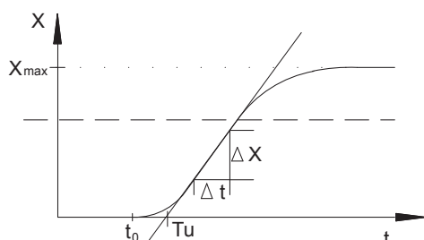
Fig. 7: Step response of a controller to a change in control variable Y. (X = actual value; e.g. disinfection or pH value)
