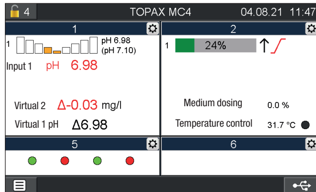
Fig. 46: Individual second overview
