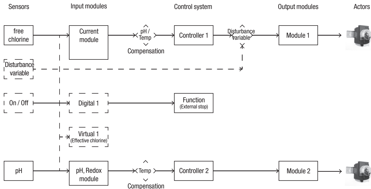
Fig. 5: Functional diagram of a two-channel controller
