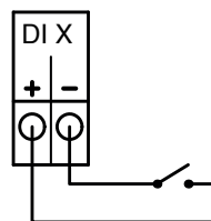
Fig. 39: Sample water shortage, external stop, medium dosing, setpoint changeover, fault indication optocoupler pump, further digital signals
