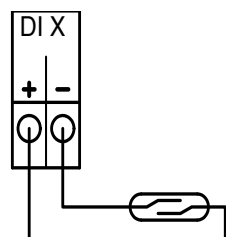
Fig. 36: Suction line, level control – 1 level, 1 cable
