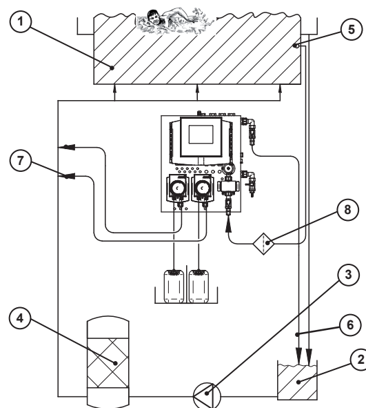
Fig. 11: Functional diagram of a swimming pool water system with an overflow channel
