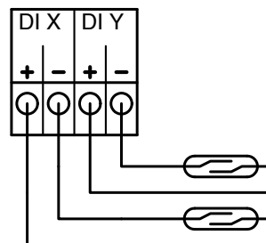
Fig. 38: Suction line, level control – 2 levels, 2 cable
