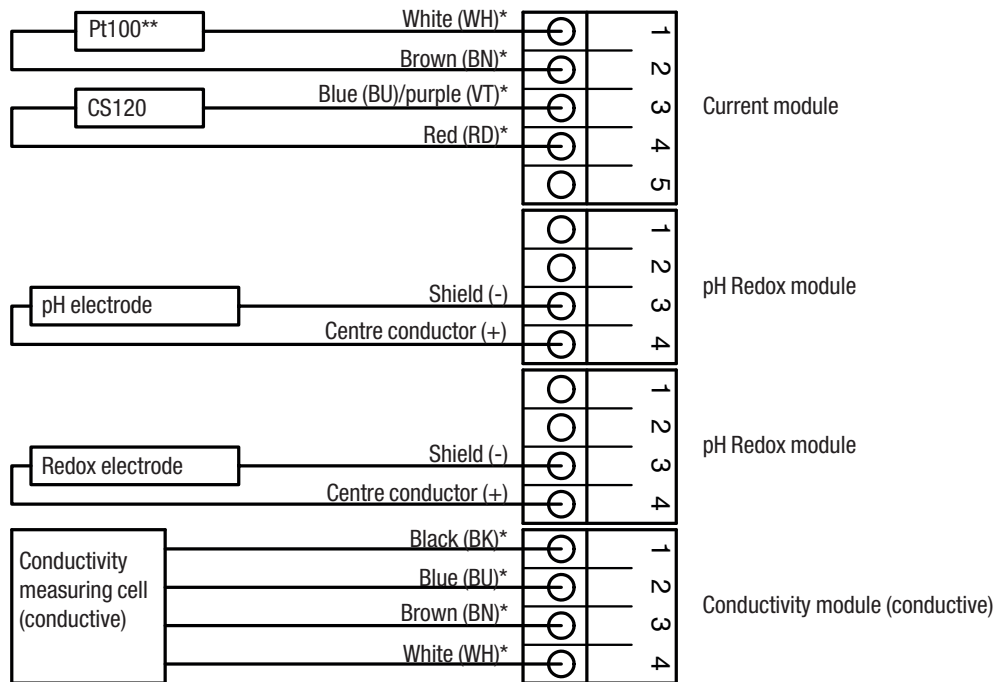
Fig. 21: Measurement of temperature, free chlorine with CS120, pH value, Redox value and conductive conductivity
