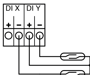
Fig. 37: Suction line, level control – 2 levels, 1 cable
