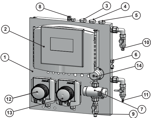
Fig. 1: Water sampling station EASYPRO SMART
