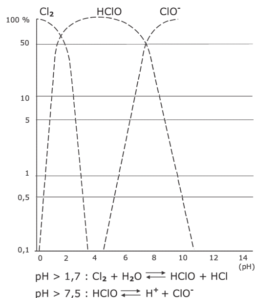
Fig. 45: Dissociation curve of free chlorine
