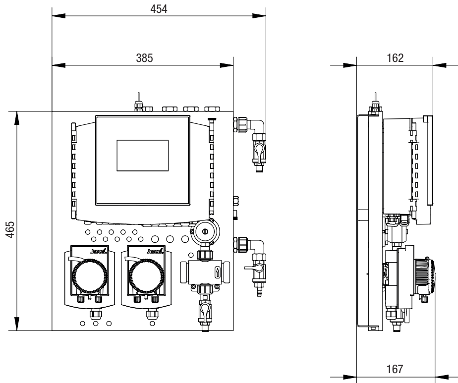
Fig. 9: EASYPRO SMART CP, CPL (with peristaltic pump and chlorine measuring cell)
