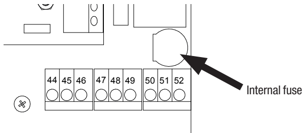
Fig. 52: Position of the fuse
