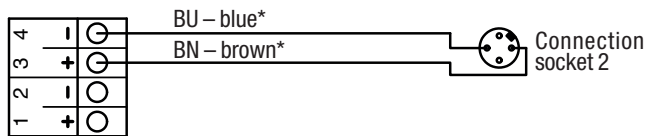
Fig. 28: Output module optokoppler, pulse frequency
