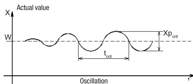
Fig. 8: Adjusting using the oscillation method:
