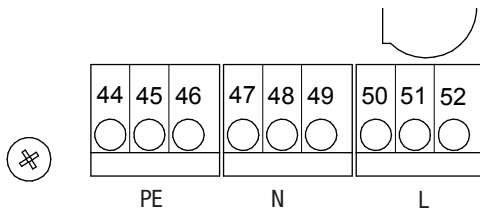
Fig. 14: Connecting the voltage supply
