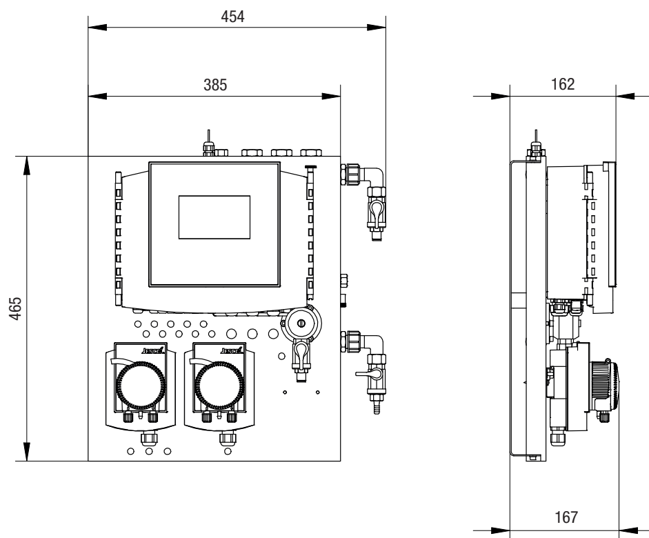
Fig. 10: EASYPRO SMART RP (with peristaltic pump without chlorine measuring cell)
