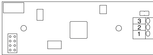
Fig. 24: Output circuit board with servomotor 20 mA
