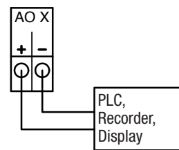
Fig. 33: Measurement outputs – measurement output/recorder outputs 4 – 20 mA, freely-configurable
