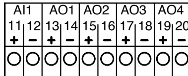
Fig. 31: Wiring diagram analogue input 11/12 and analogue outputs 13 – 20
