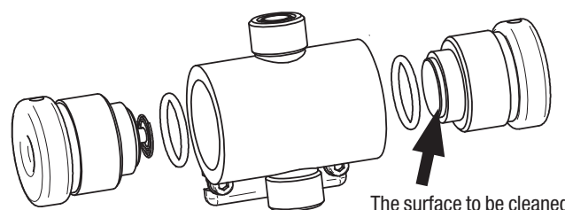
Fig. 47: Chlorine measuring cell
