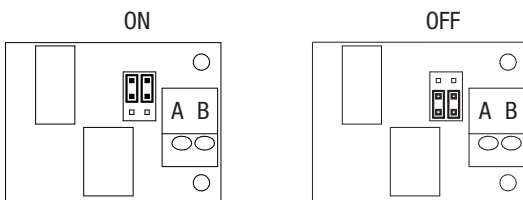
Fig. 41: Jumper position on RS485
