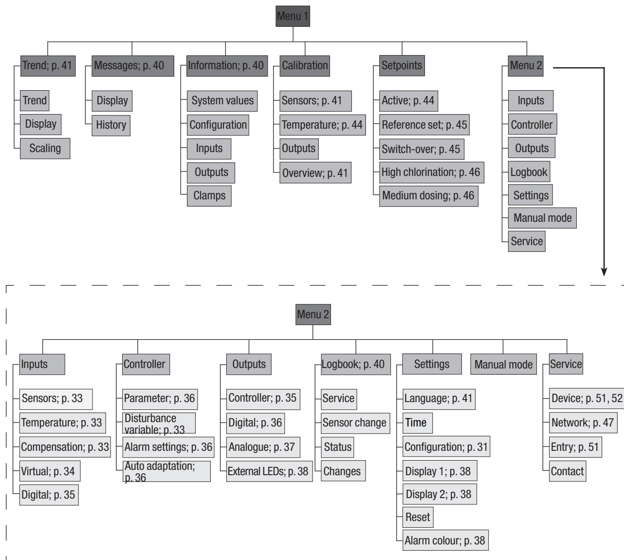
Fig. 42: Menu structure of TOPAX®
