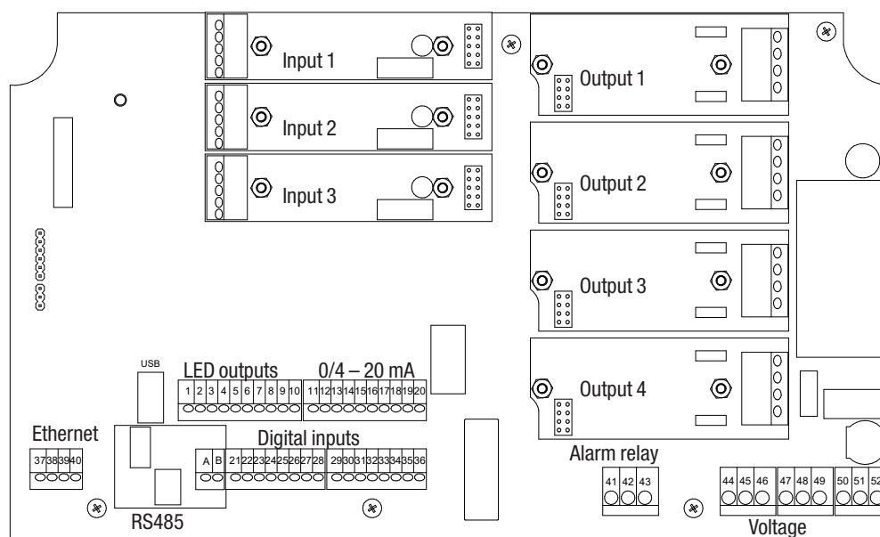
Fig. 15: Overview of the connection clamps
