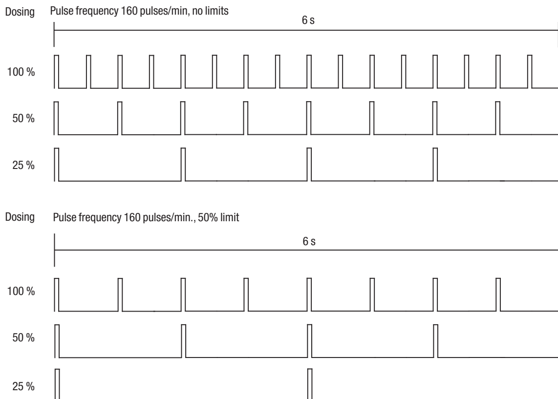
Fig. 44: Function of the pulse frequency e.g. for MAGDOS pumps
