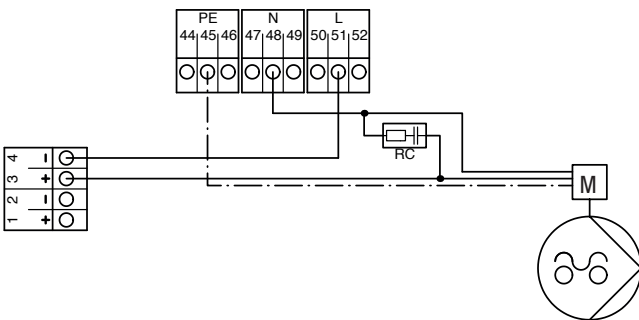
Fig. 30: Peristaltic pump 2.7 l/h (output module relay/relay high current, pulse length)
