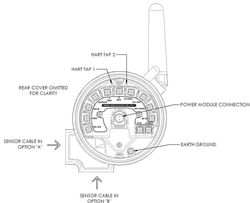
Figure 3-1. Sensor Wiring & Connection Points for 6081
