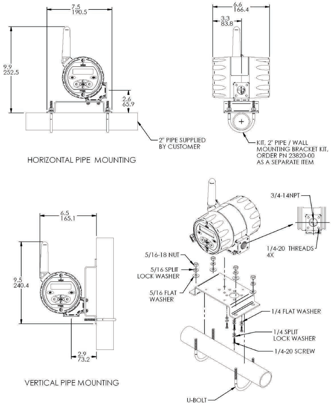
Figure 2-2. Pipe Mounting Installation Model 6081. Use Pipe/Wall Mounting Bracket Kit, PN 23820-00
