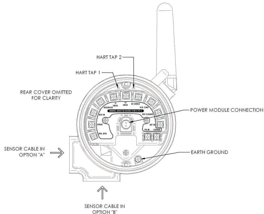
Figure 7.1. 6081 Sensor Wiring & Connection Points
