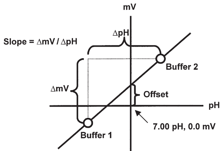
Figure 10-1. Calibration Slope and Offset
