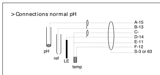
Figure 3-11b. Sensor wiring
