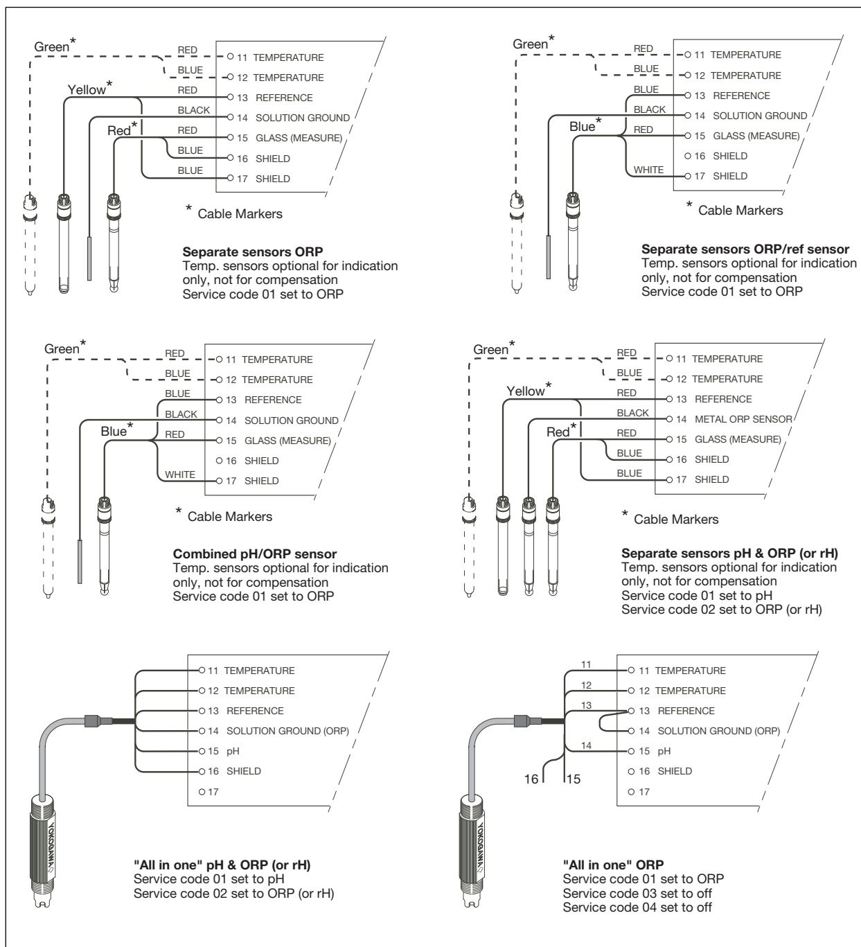
Figure 3-11b. Sensor wiring
